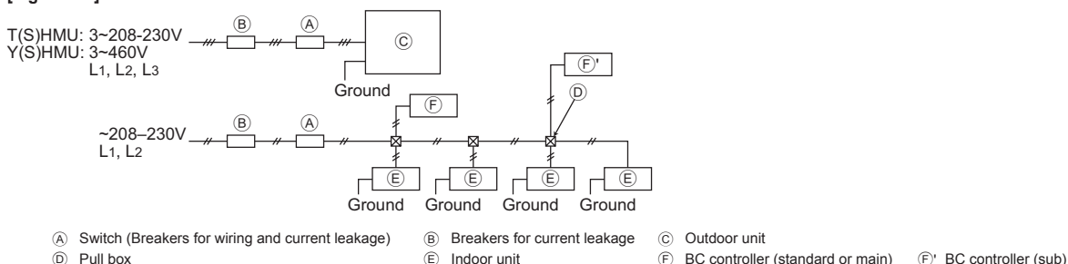
Thickness of wire for main power supply, ON/OFF capacities
