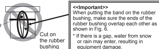
<Fig. 7: Back of the rubber bushing>
