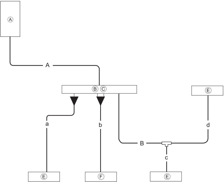
[Outdoor model: P144YSKMU, P168~ P288T/YSKMU]
