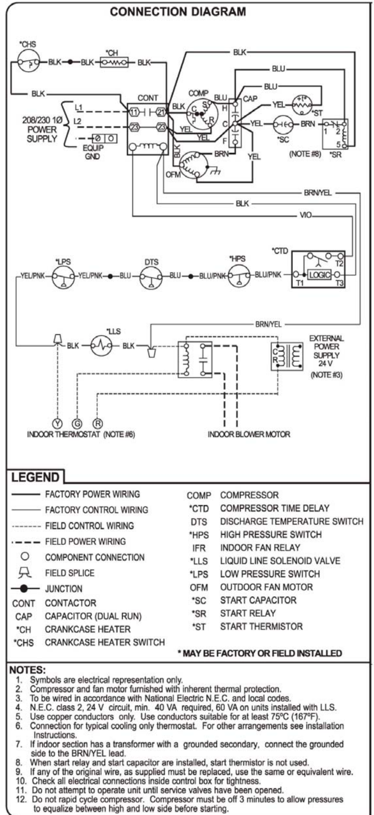
Figure 4 - Cooling Only
