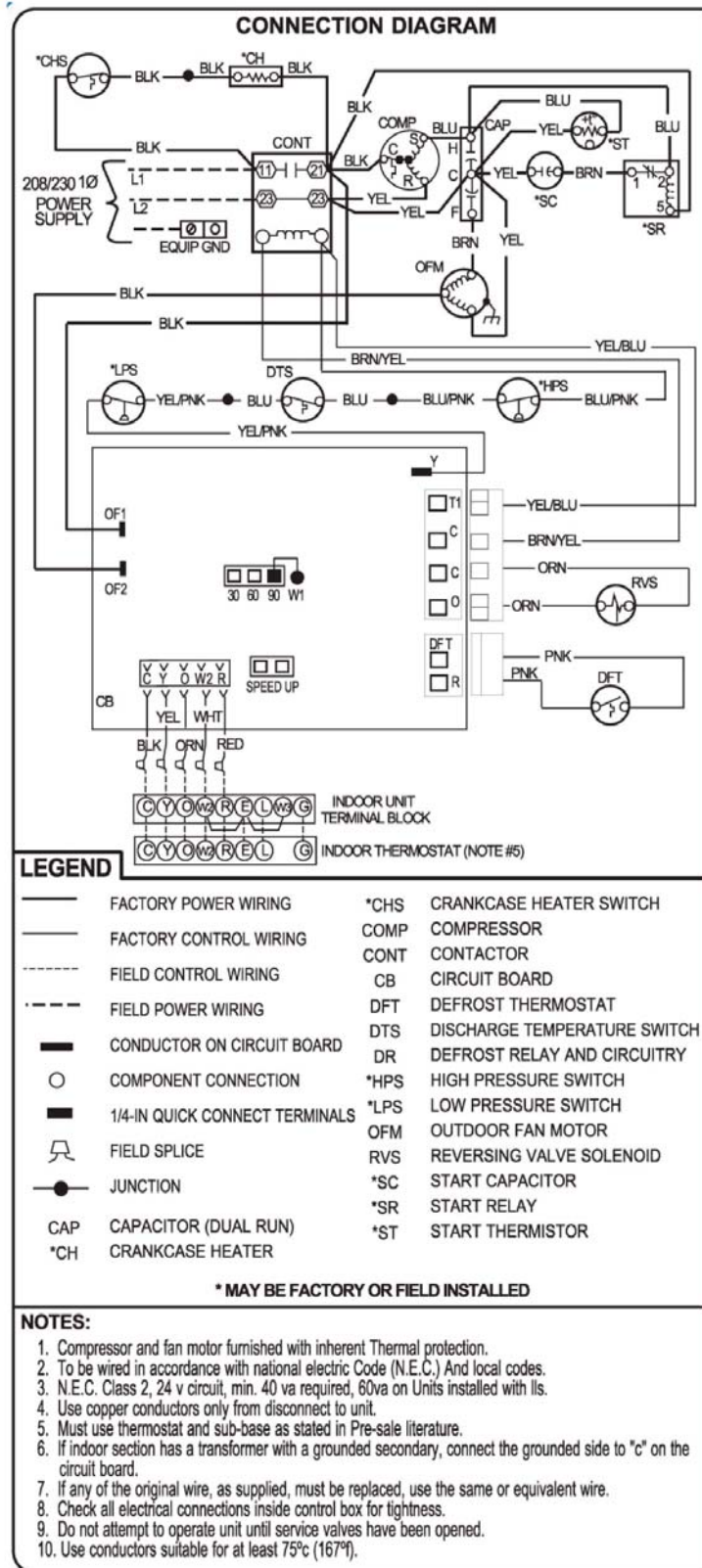
Figure 3 - Heat Pump
