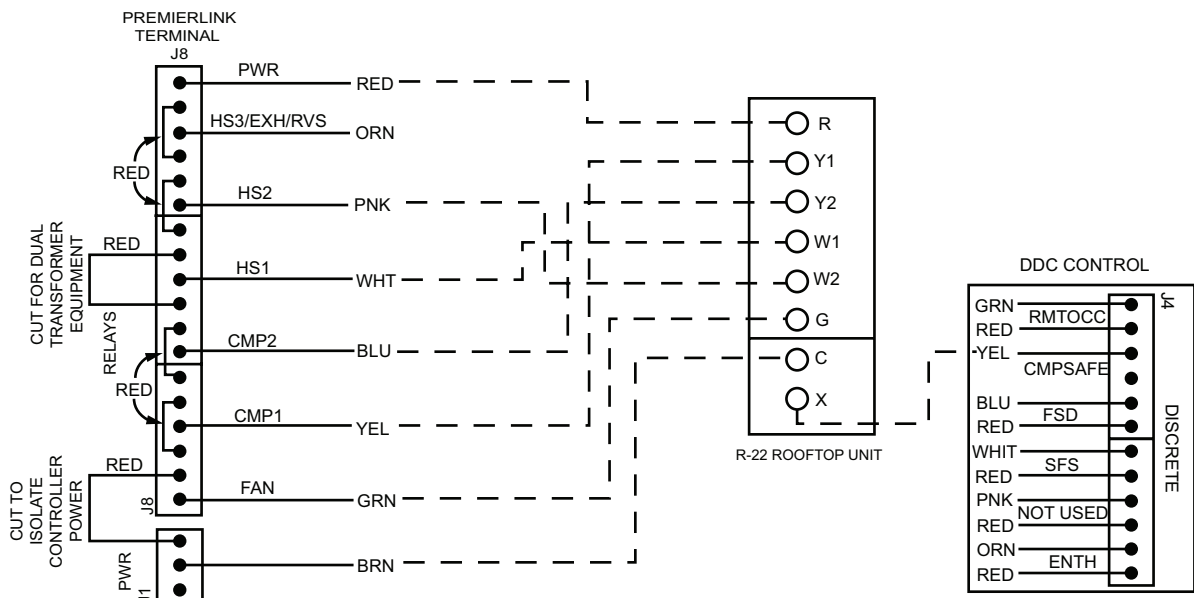
Figure 10 - Typical PremierLink Control Wiring To Rooftop R-22 Units
