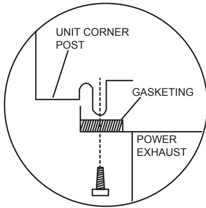
Figure 11 - Gasketing Location Detail (Standard Filter Panel Only)
