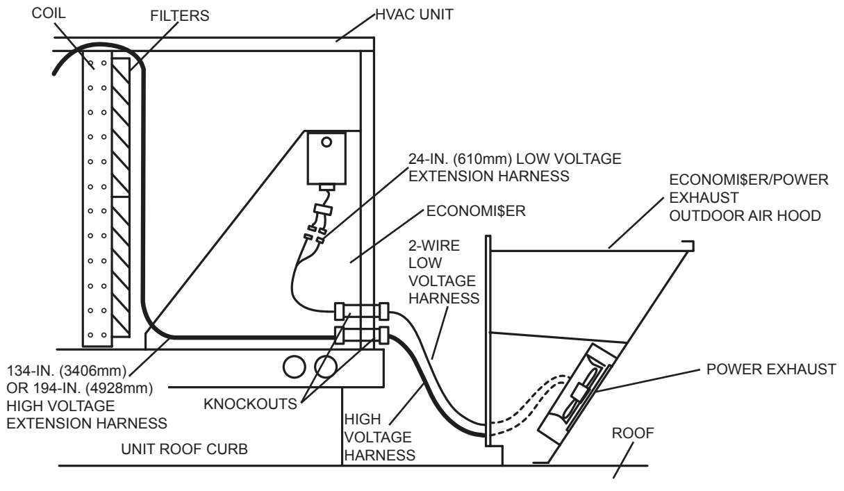
Figure 5 - Power Exhaust Harness Installation for EconoMiSer X with W7220 Controller
