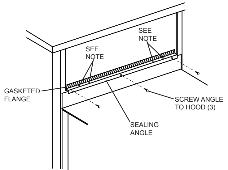
Figure 15 - Install Sealing Angle
