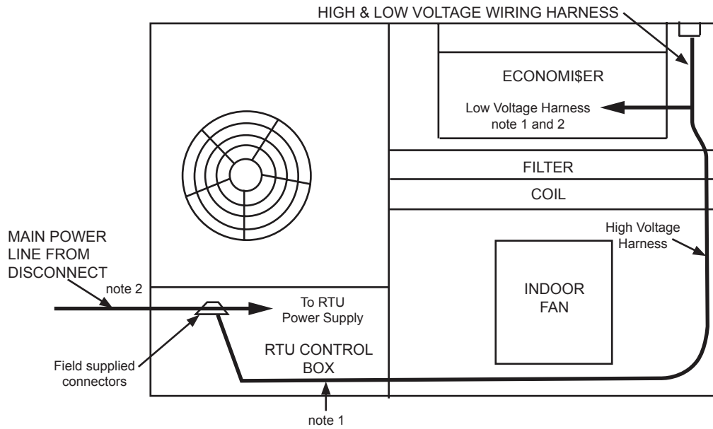
Figure 6 - Power Line Harness Routing (Top View of Unit Shown)
