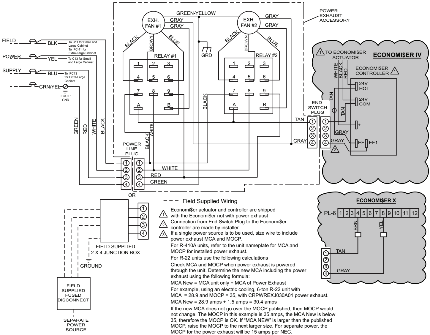
Figure 8 - Power Exhaust Wiring for EconoMiSer IV and EconoMiSer X with Controller W7212-460 V Units
