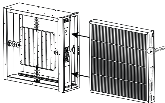
Fig. 16 - Replace Filter
