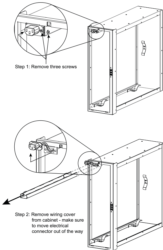
Fig. 9 - Removal of Electrical Tray Cover
