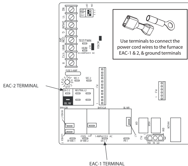
Fig. 12 - Air Purifier Connection to Furnace
