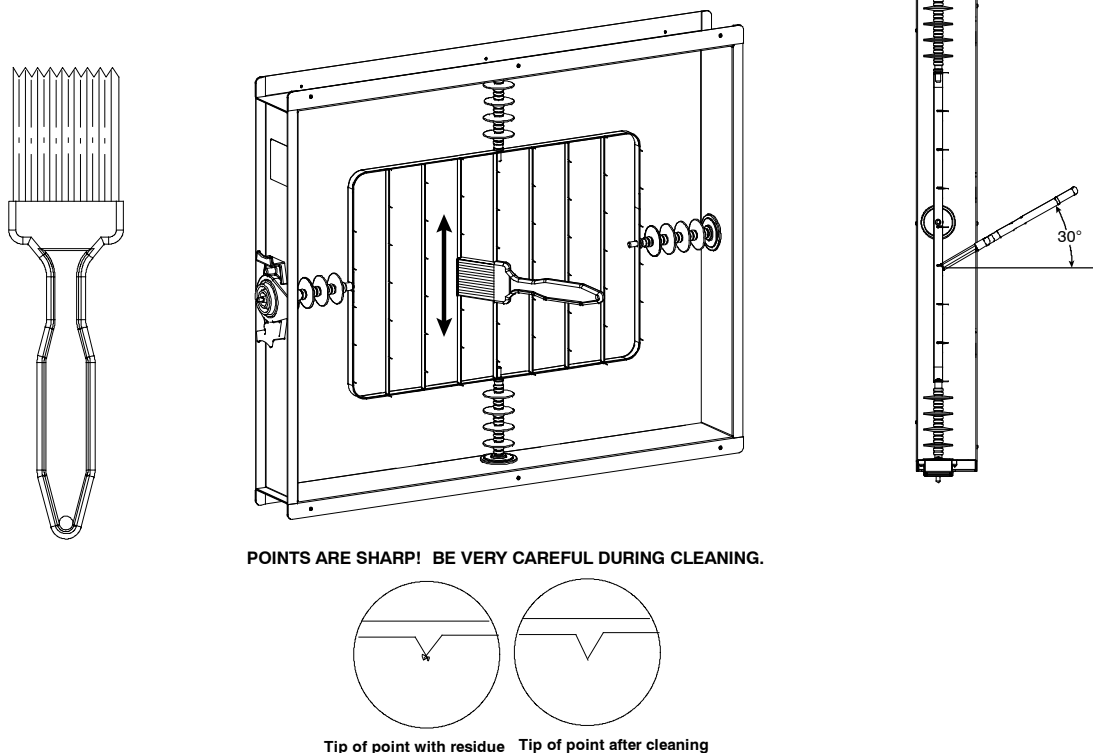
Fig. 19 - Removal of Deposits from Ionization Pins
