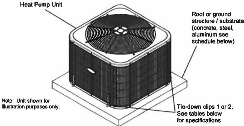
TIE-DOWN CLIP (1) (GROUND AND ROOF APPLICATION)
