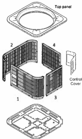
Note: Image is not to scale and is for illustration purposes only. Actual units may differ slightly in appearance. Cabinet 226CN Cabinet 126CN
