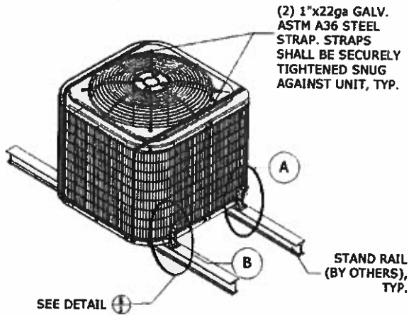
1 MECHANICAL UNIT N.T.S. FRONT ISOMETRIC
