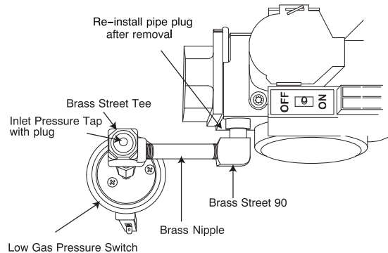
Fig. 12 - Alternate Low Gas Pressure Switch - 17 1/2-in and Wider Furnaces
