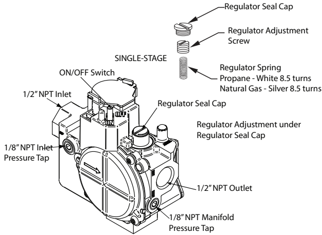
Fig. 10 - Single-stage valve
