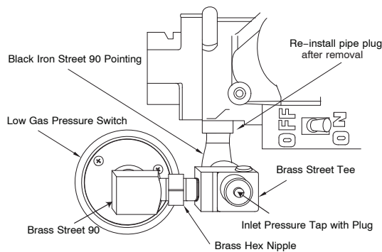
Fig. 11 - Low Gas Pressure Switch - All Widths
