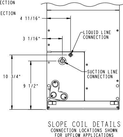
Fig. 1 - FY5B Dimensions - English
