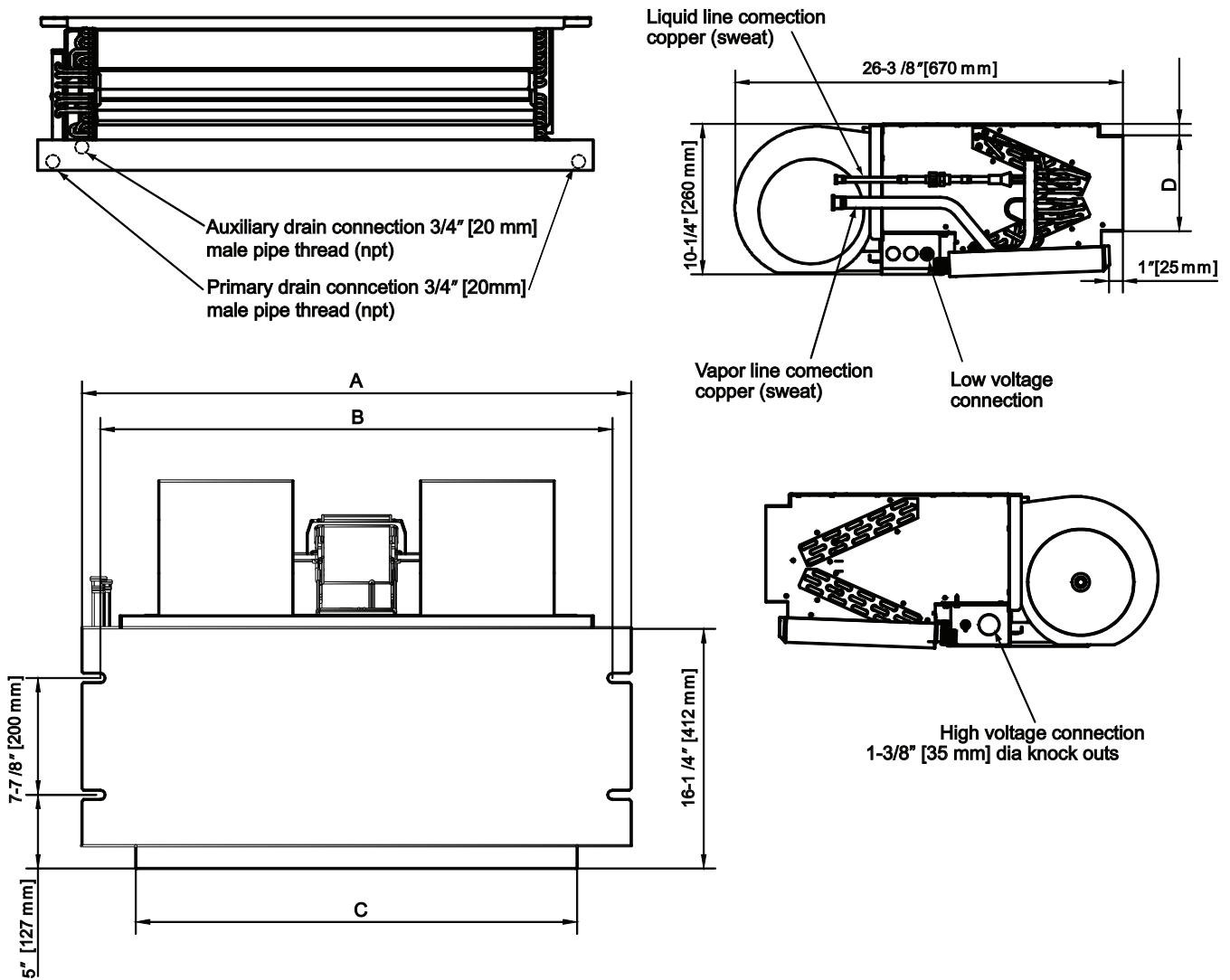
Fig. 3 - FPM(A,B)NU Uncased Horizontal Fan Coil Dimensional Drawing (FPMANU model shown)
