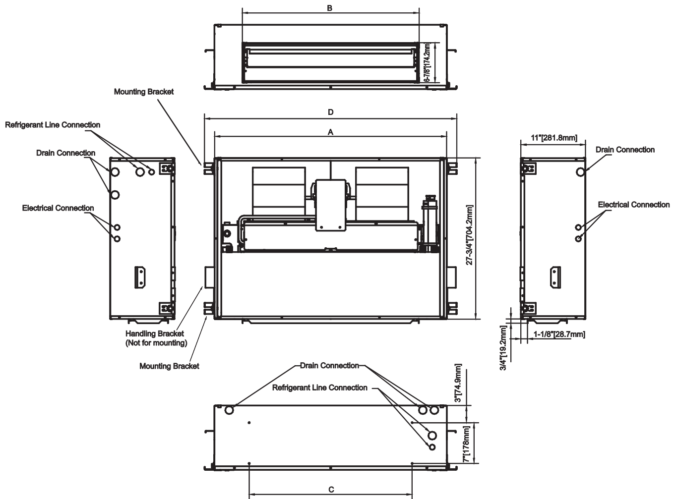
Fig. 4 - FPM(A,B)NC Cased Horizontal Fan Coil Dimensional Drawing (FPMANC model shown)
