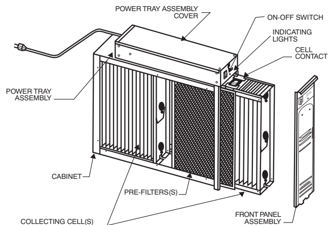
Fig. 1 - Unit Assembly
