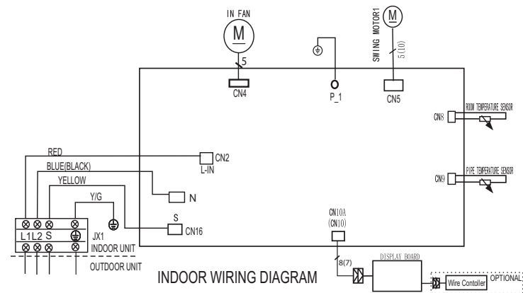
Fig. 14 – Wiring Diagram Size 30 and 36 (208–230V)
