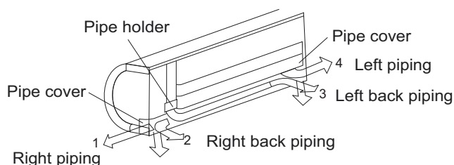
Fig. 7 – Piping Locations
