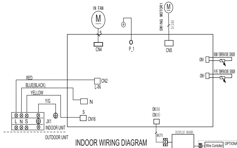
Fig. 10 – Wiring Diagram Sizes 09–12 (115V)
