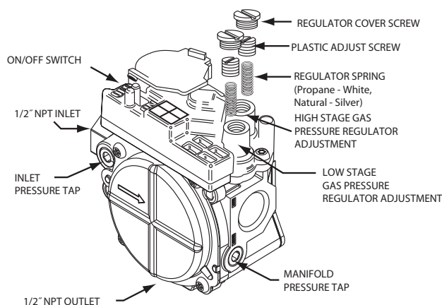
Two-Stage 36G Valve
