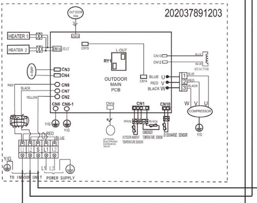
Indoor unit Outdoor unit CODE PART NAME CODE PART NAME CN1 Input: 230VAC High voltage Connection of the terminal CN7、CN8 Input: 230V High voltage CN3 Output: 0-5VDC Connection of the CCM CN2 Output: Connection of the high voltage P1 Output: 0V Connection of the earth CN3、CN4 Output: High voltage for 4-way control CN5 Output: 1-5VDC Connection of the Water level switch CN11、CN16 Output: 230V High voltage for HEATER CN6 Output: 5VDC Connection of the Room and Pipe temperature CN5 Output: Pulse(0-320V) for DC FAN CN10A Output: 12VDC Connection of the Display board CN12、CN13 Output: Connection of the high voltage CN13 Output: 220VAC High voltage Connection of the Pump U V W Output: Pulse(0-320V) for compressor CN14 Output: 12VDC Connection of the Swing motor CN10 Input:Pin1 (5V) Pin2(0-5V) CN15 Output: 320VDC High voltage Connection of the DC Fan CN1 Input:Pin3-4 (5V) Pin2(0V),Pin1,Pin5(0-5V) CN16 Output: 320VDC High voltage Connection of the Reactor CN18 Output:Pin5&6(12V) Pin1-Pin4:Pulse waveform,(0-12V) CN23 Output: 1-12VDC Connection of the Remote switch CN33 Output: 0V Connection of the Alarm CN40 Output: 12VDC Connection of the Wire controller CN110 Output: 24VDC Between Pin2 of CN1 Connection of the S signal
