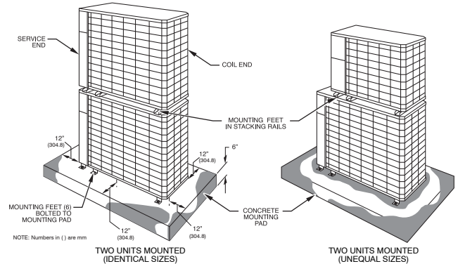
Fig. 3 – Stacking Kit
