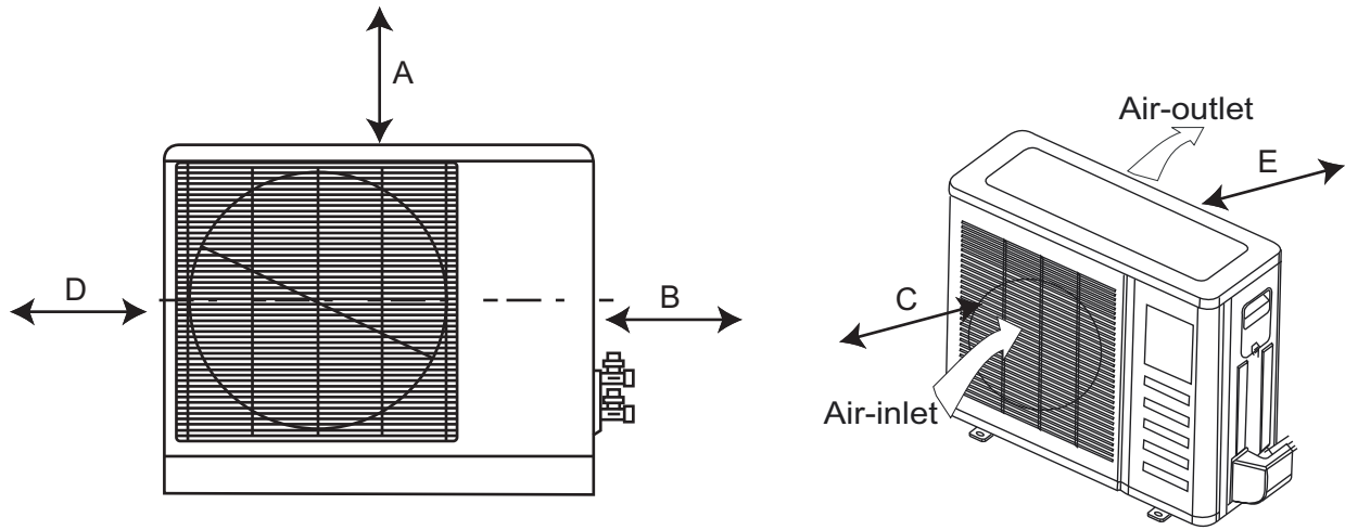
Fig. 8 – Outdoor Unit Clearance
