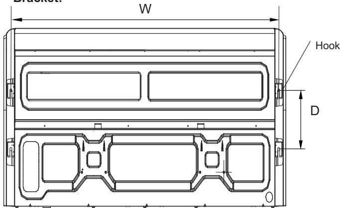
Fig. 5 – 40MKCB**F, 40MKQB**F Unit and Bracket Dimensions
