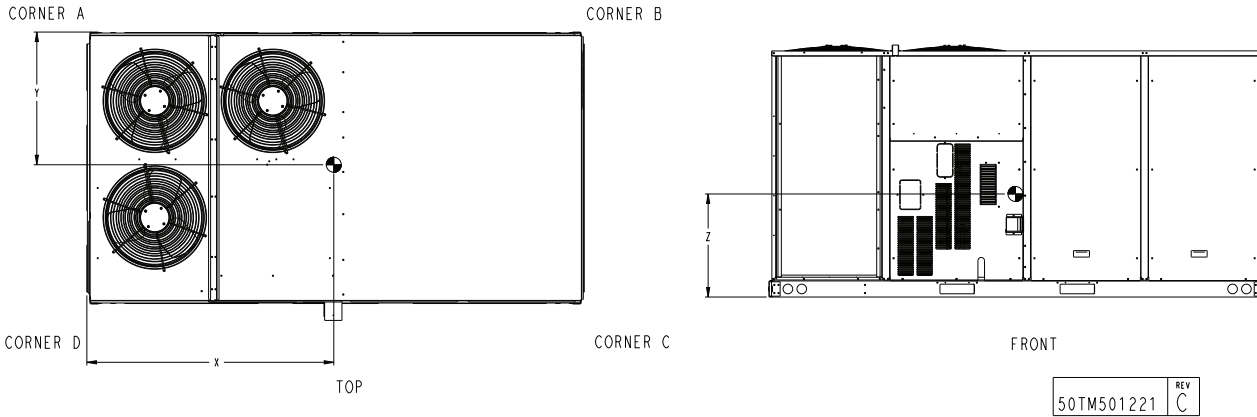
Fig. 13 - Dimensions 48TC 16
