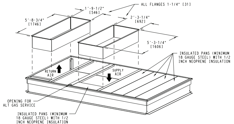
Fig. 7 - Roof Curb Details – 21 and 25 Size Units
