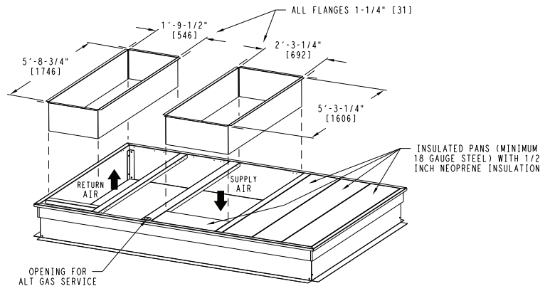
Fig. 6 - Roof Curb Details - 18 Size Unit
