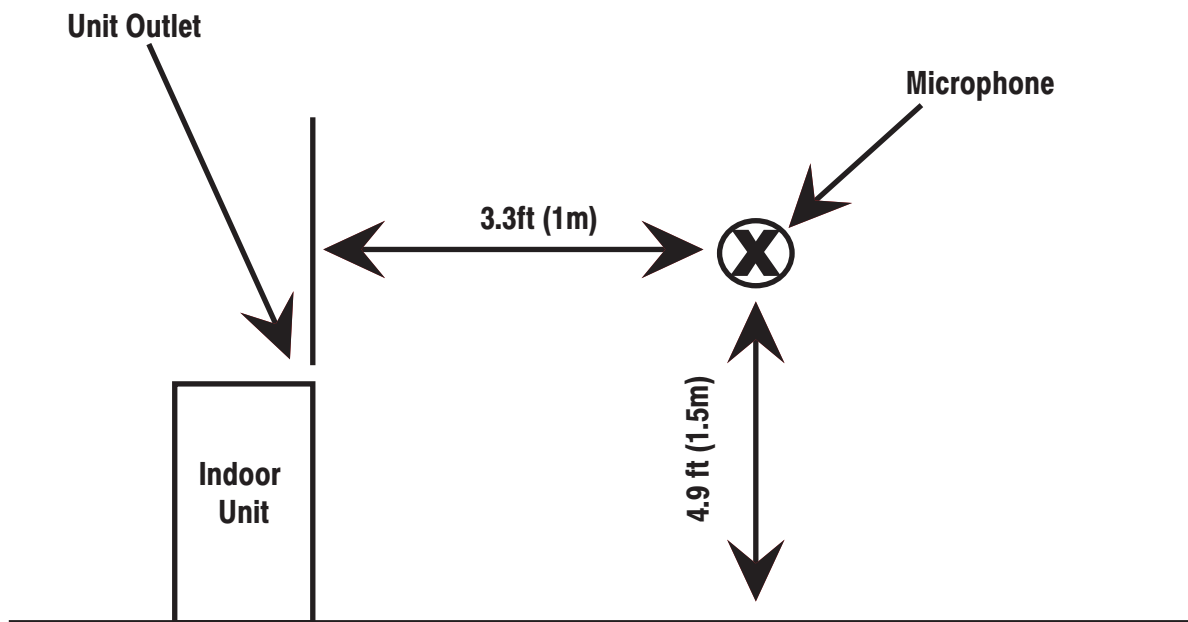
Fig. 7 – Sound Pressure Testing Method
