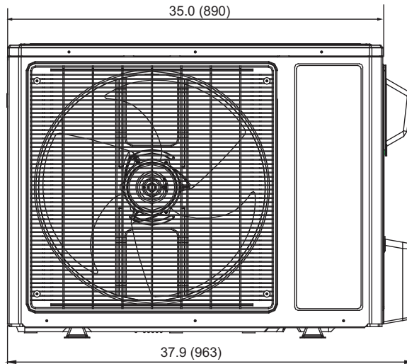
Fig. 4 – 12K 230V (Net Operating Weight: 63.8 lbs. / 30 kg)
