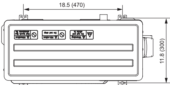
Fig. 4 – 12K 230V (Net Operating Weight: 63.8 lbs. / 30 kg)
