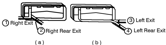
Fig. 8 – Refrigerant Line Routing
