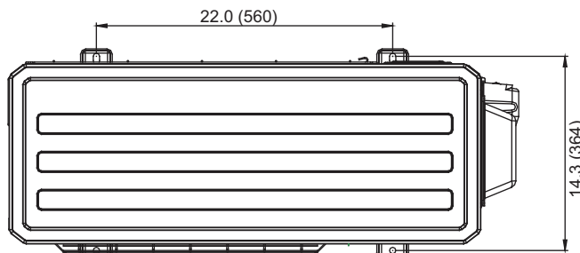
Fig. 5 – 18K and 24K (Net Operating Weight: 112.2 lbs. / 51 kg)
