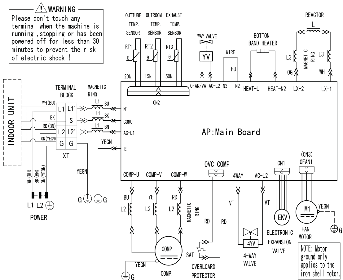
Fig. 14 – Outdoor unit
