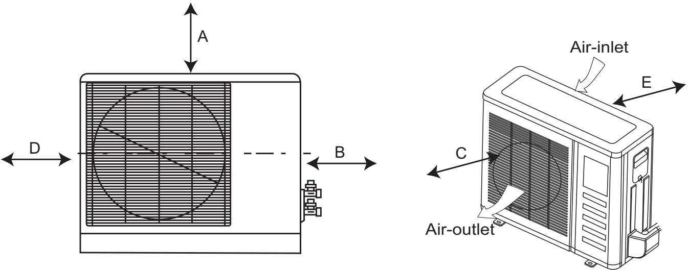
Fig. 6 – Clearances Outdoor
