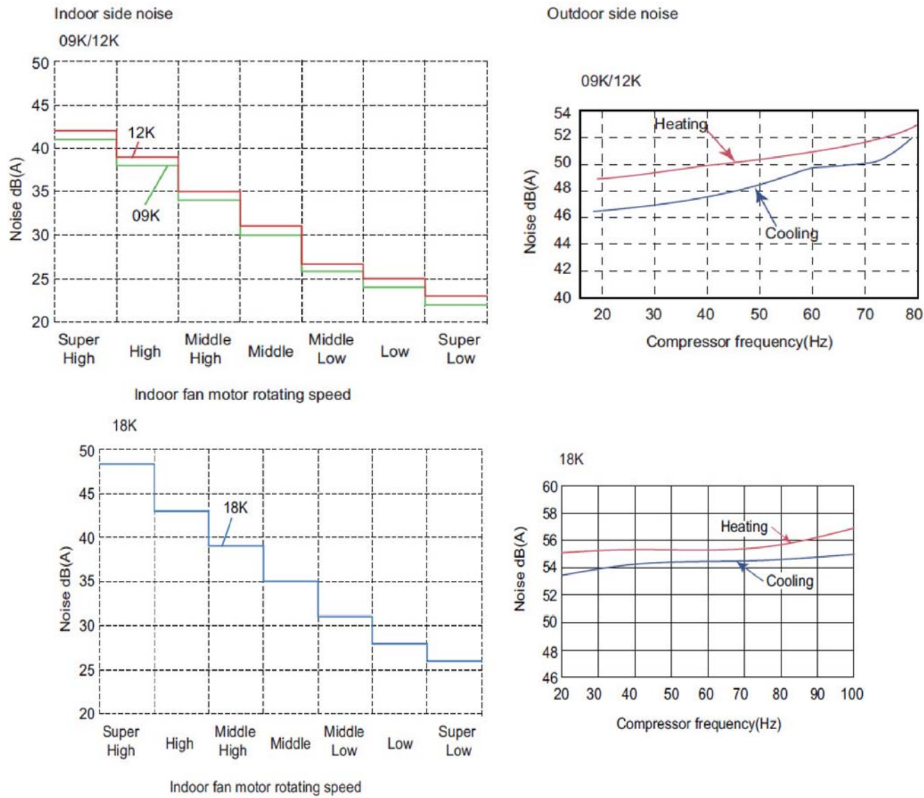
Fig. 10 – Sound curve
