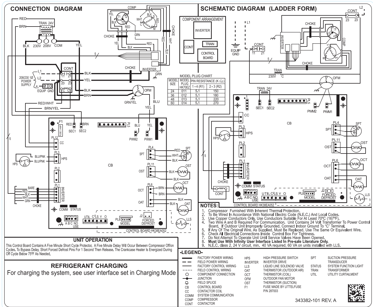
Fig. 1 – Wiring Diagram — 24VNA0 Model sizes 2 - 5 tons, 208/230-1
