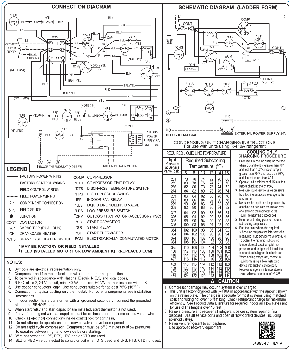
Fig. 3 – Wiring Diagram — Model BA16NW061, 208/230-1
